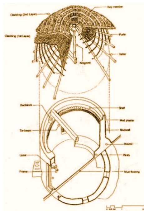
Fig. 10. Exploded view of construction detail (Source: Lathiya, 2016)
